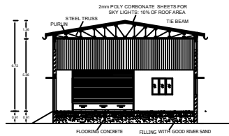
SECTION ON "MS"
