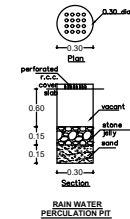
RAIN WATER PERCOLATION PIT
