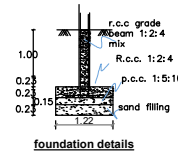
foundation details
