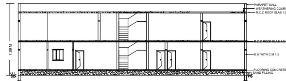
SECTION ON S.P
