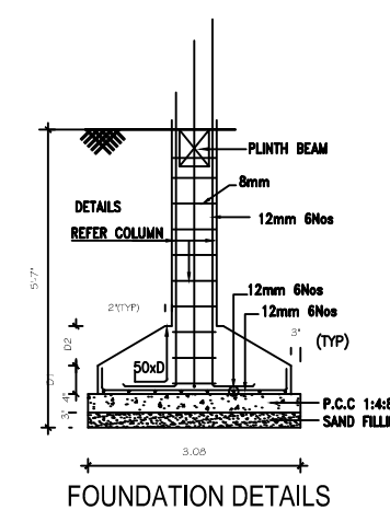
FOUNDATION DETAILS
