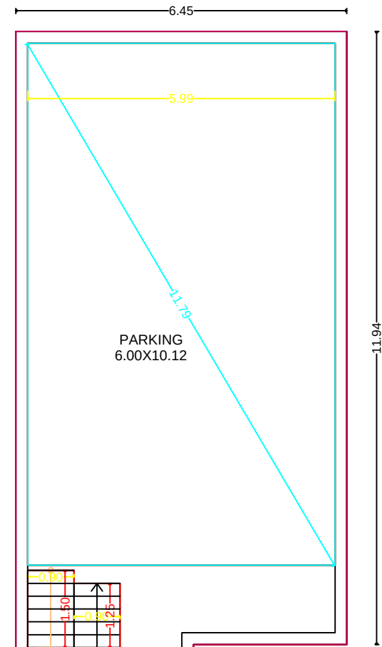
FLOOR PLAN
