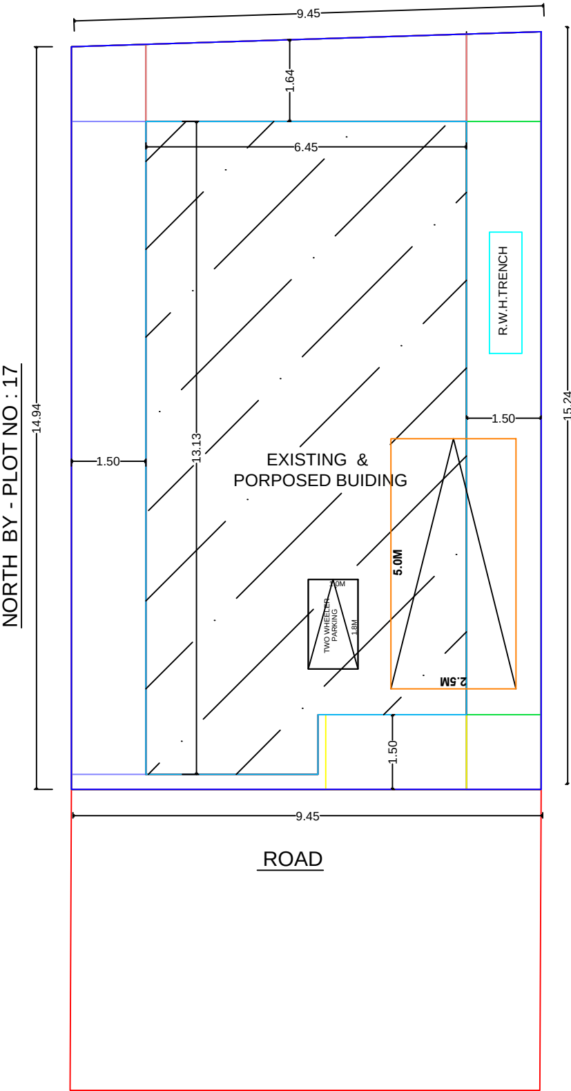
SITE PLAN
