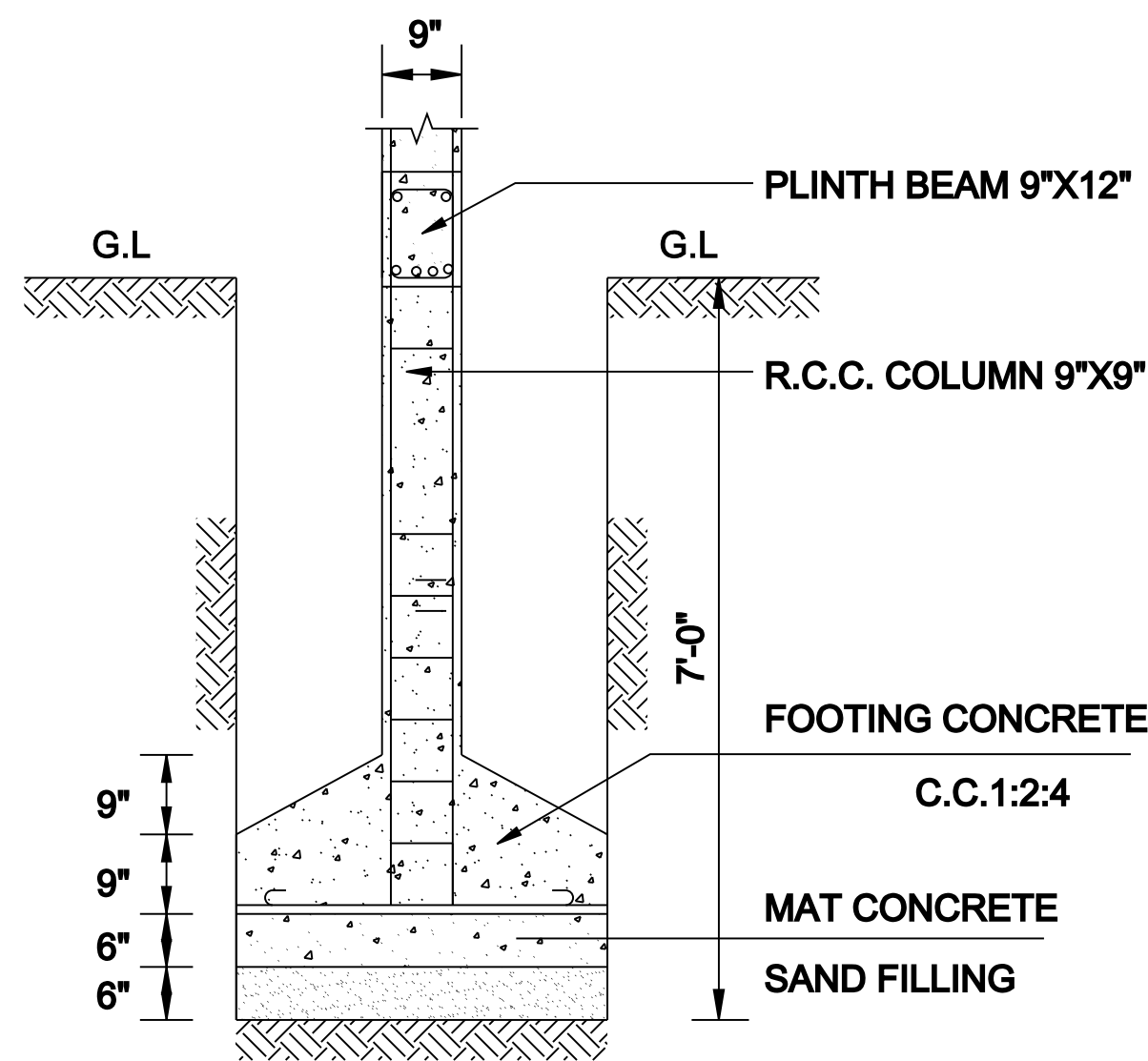
FOUNDATION DETAILS NOT TO SCALE
