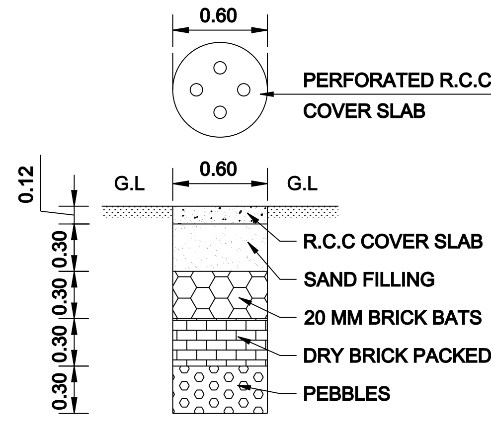
RAIN WATER HARVESTING NOT TO SCALE
