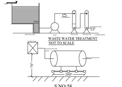
SOLAR HOT WATER SYSTEM DETAILS
