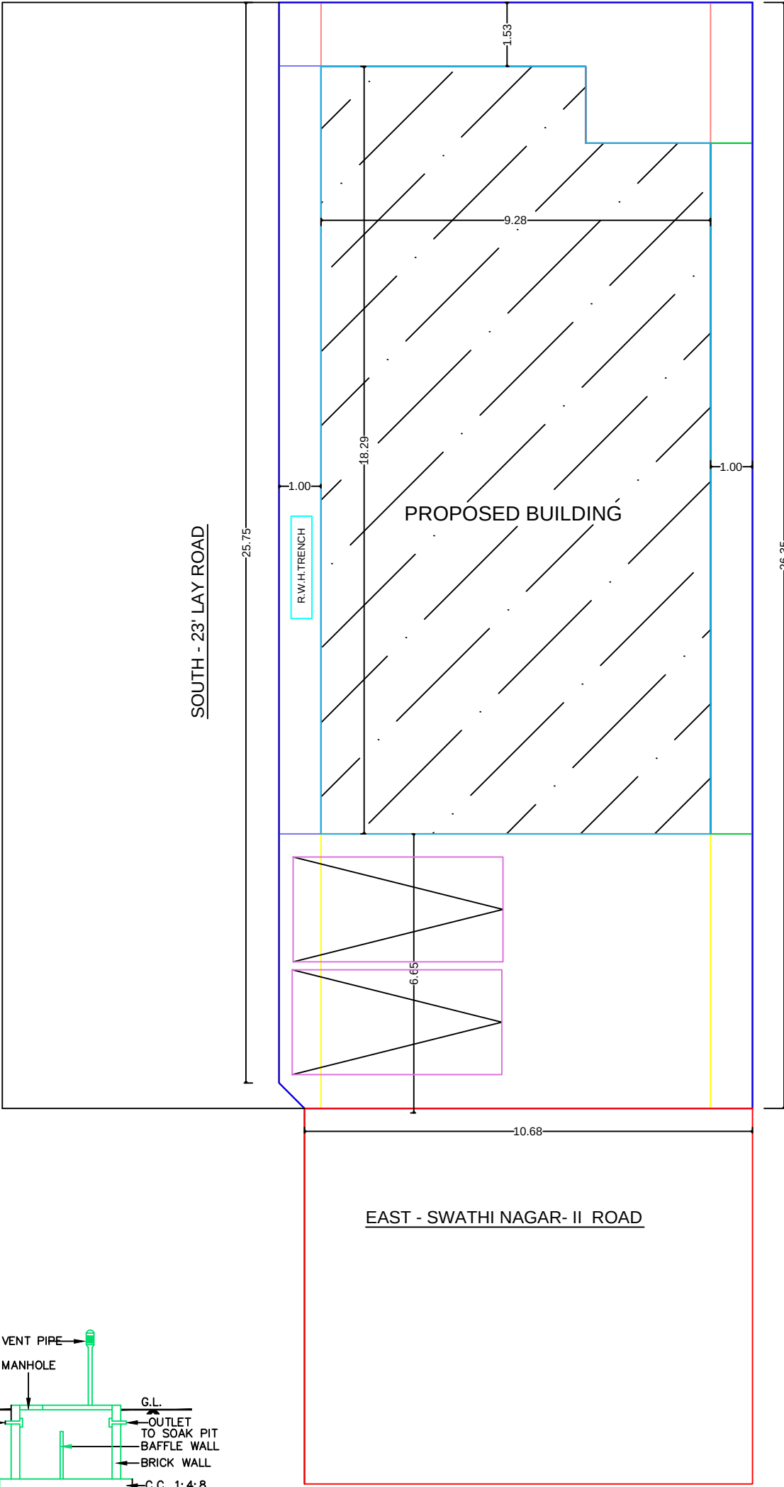
SITE PLAN
