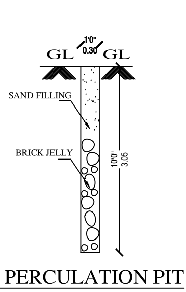
PERCOLATION PIT
