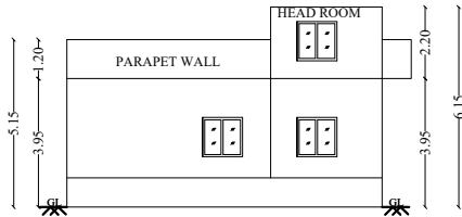
WEST SIDE ELEVATION
