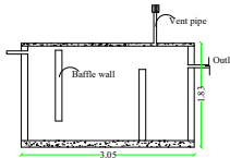
SEPTIC TANK DETAILS Size: 3.05 x 1.83 SCALE 1:100
