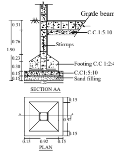
FOUNDATION DETAILS
