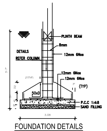
FOUNDATION DETAILS
