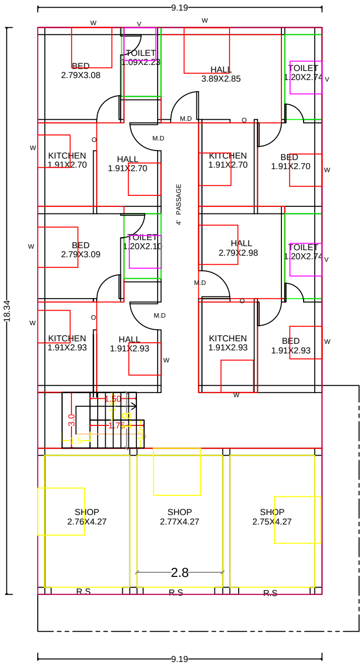
FLOOR PLAN
