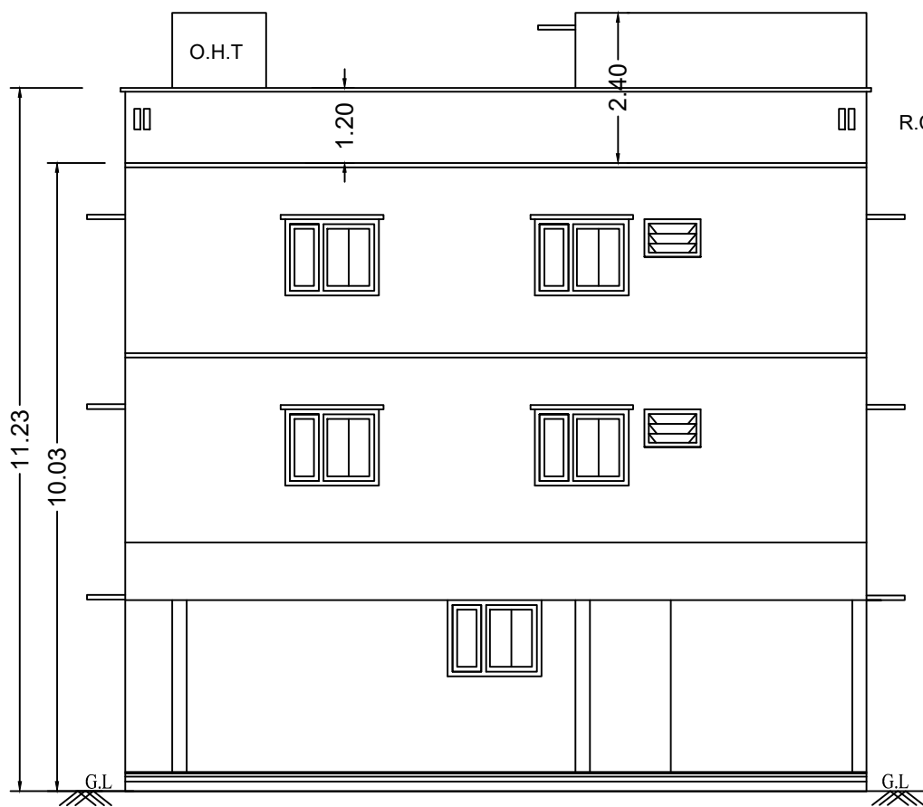
FRONT ELEVATION
