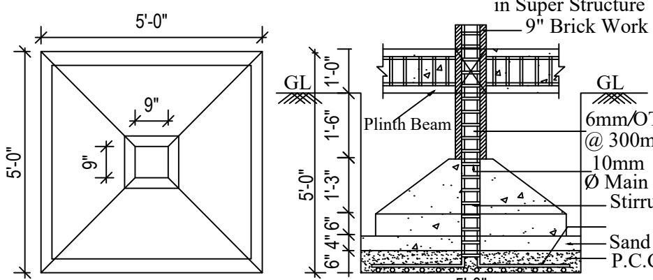
PLAN
