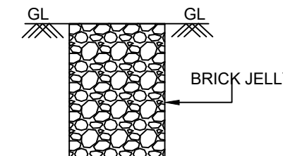
PERCOLATION PIT
