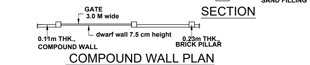
COMPOUND WALL PLAN
