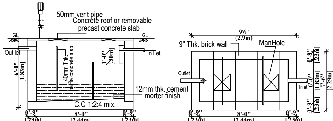
SECTION
