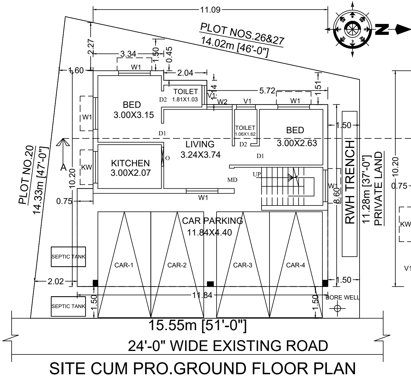
SITE CUM PRO.GROUND FLOOR PLAN
