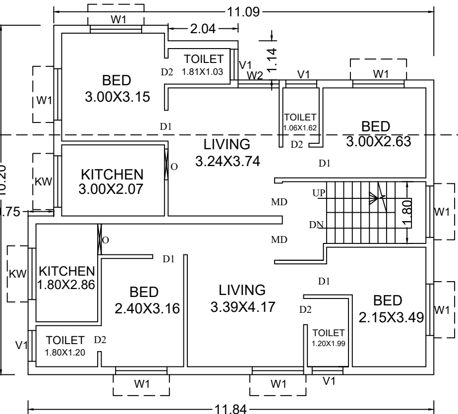
PRO.TYPICAL FLOOR PLAN [FIRST & SECOND FLOOR]
