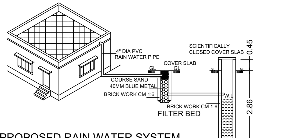
PROPOSED RAIN WATER SYSTEM WITH WELL DETAIL
