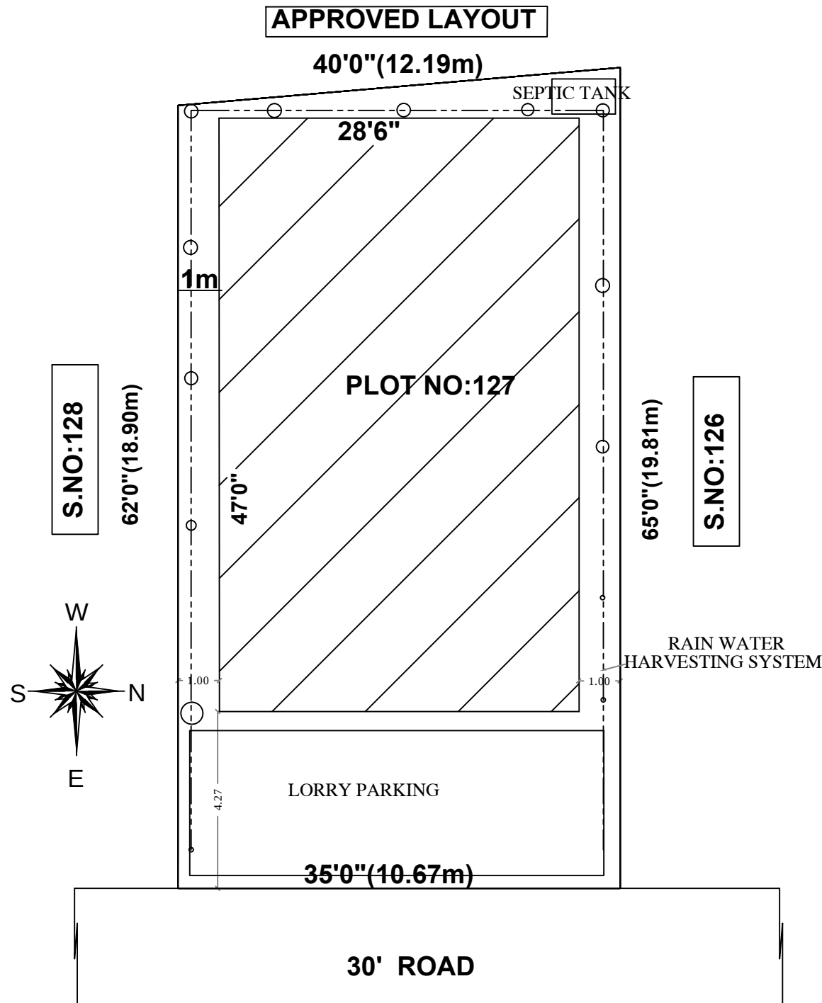
SITE PLAN
