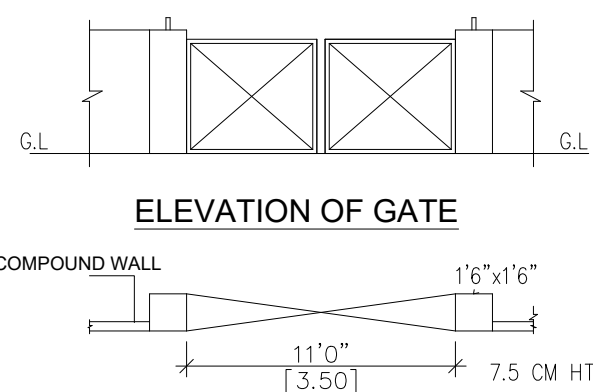
GATE & COMPOUND WALL PLAN
