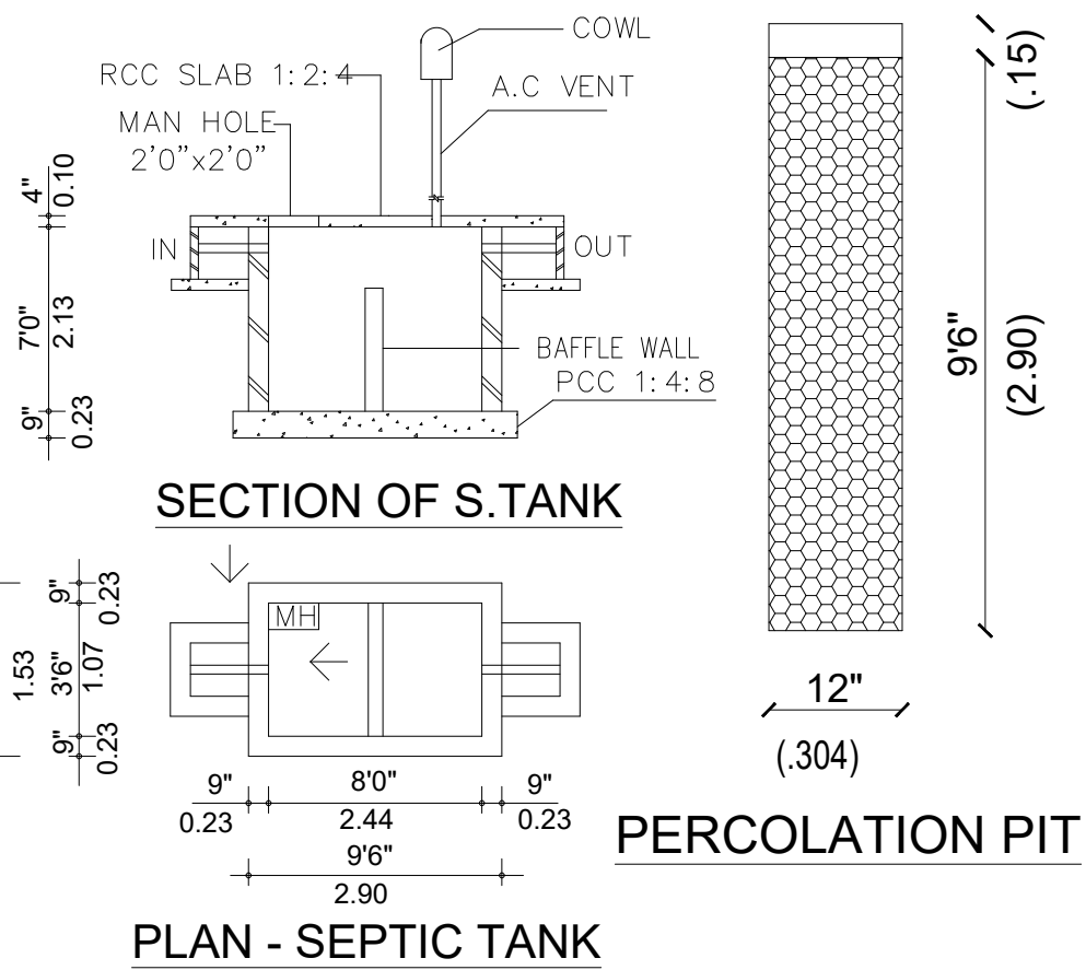
PLAN - SEPTIC TANK
