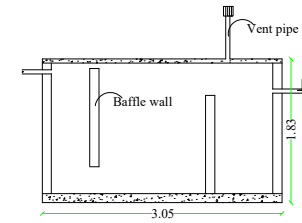
SEPTIC TANK DETAILS Size: 3.05 x 1.83 SCALE: 1:100
