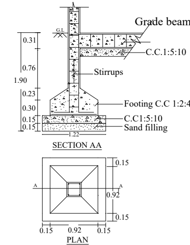
FOUNDATION DETAILS
