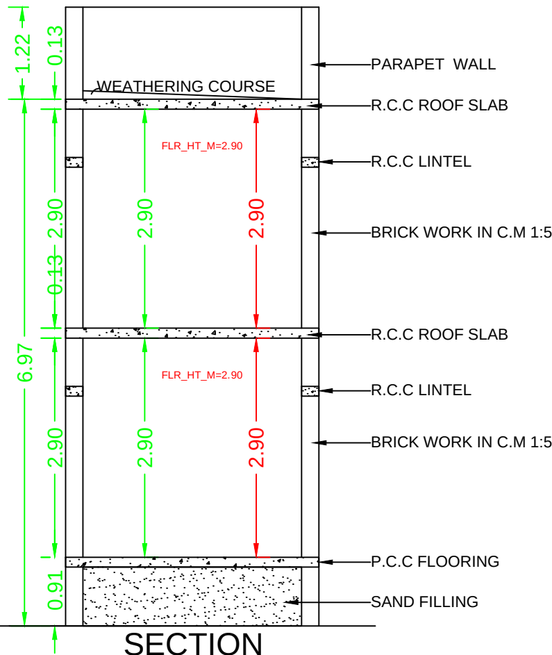
SECTION
