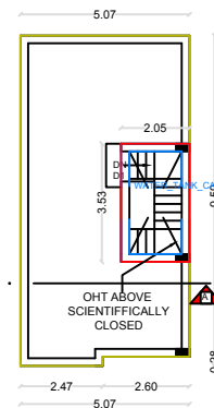
TERRACE FLOOR PLAN (PROPOSED)
