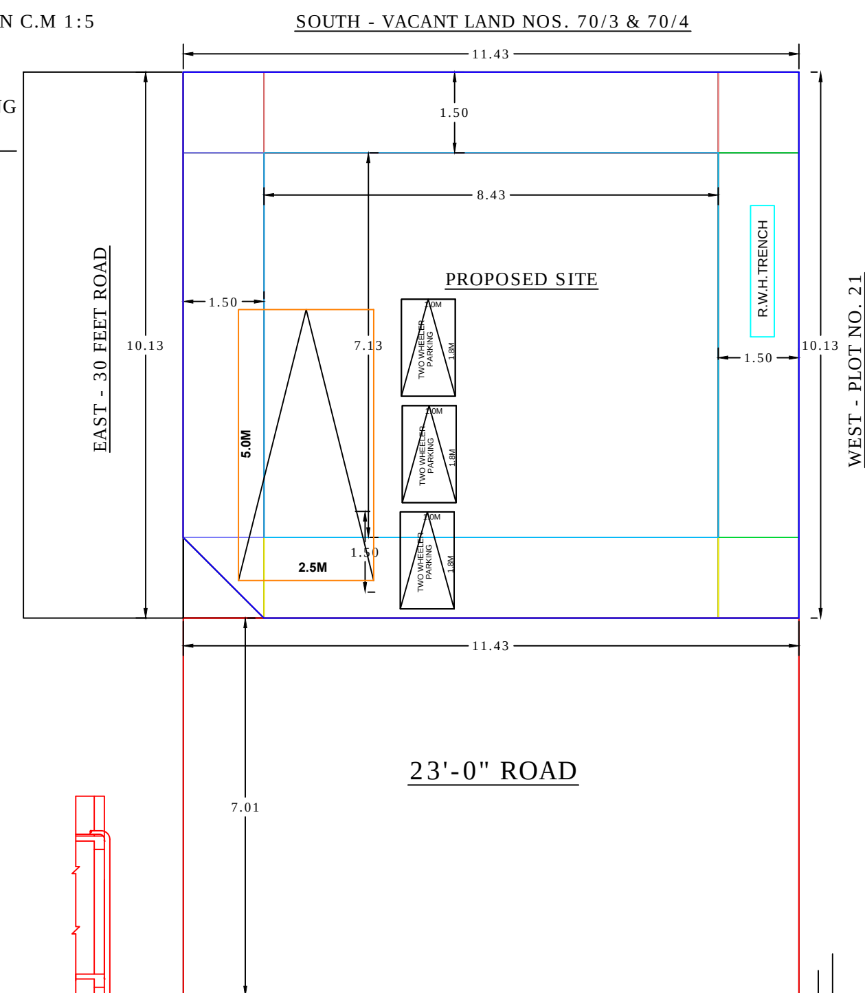
SITE PLAN
