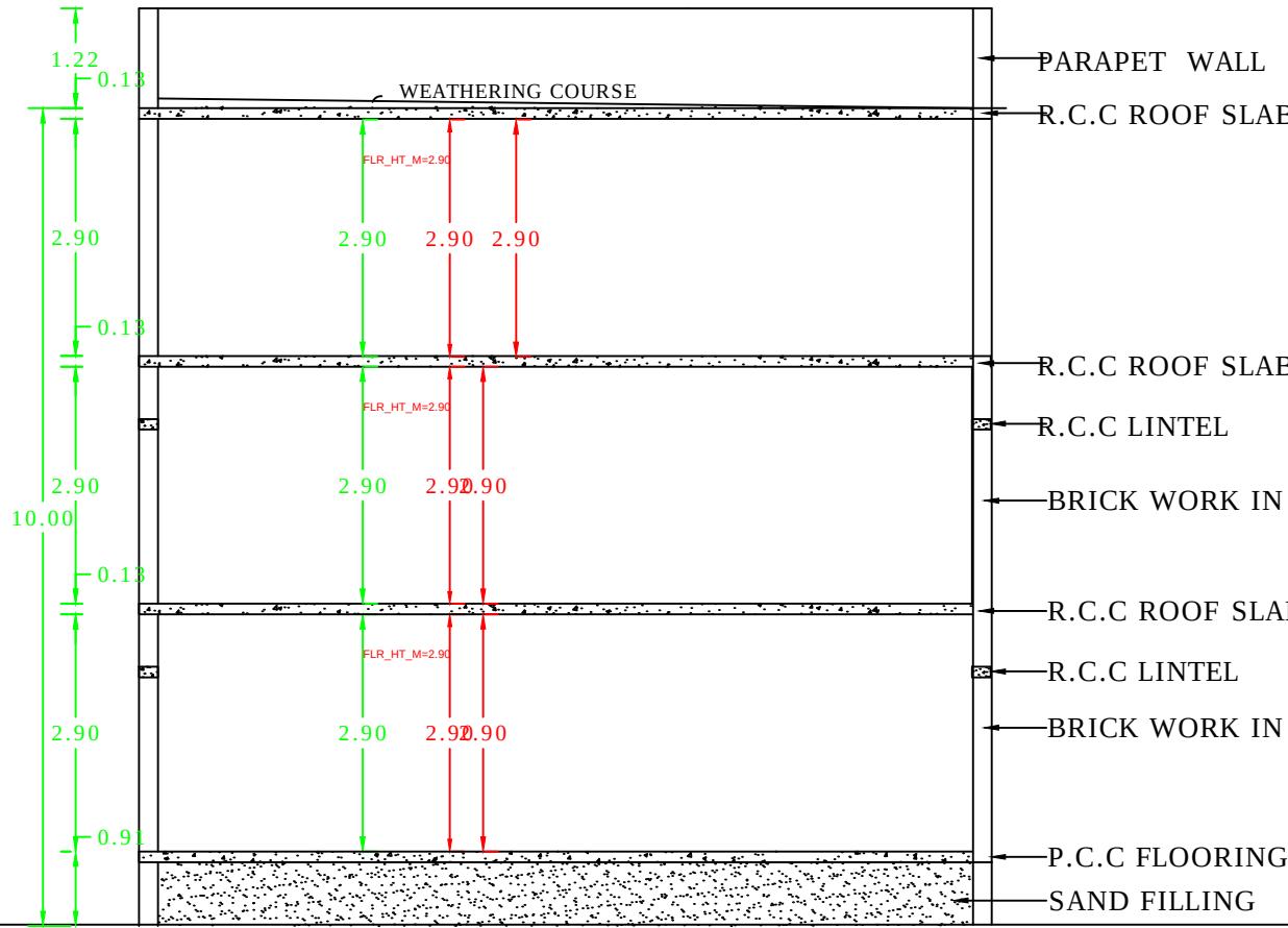
SECTION
