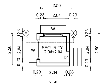
GROUND FLOOR PLAN (Security Room)
