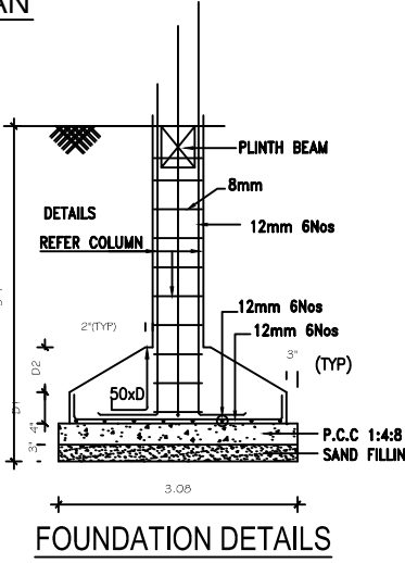
FOUNDATION DETAILS
