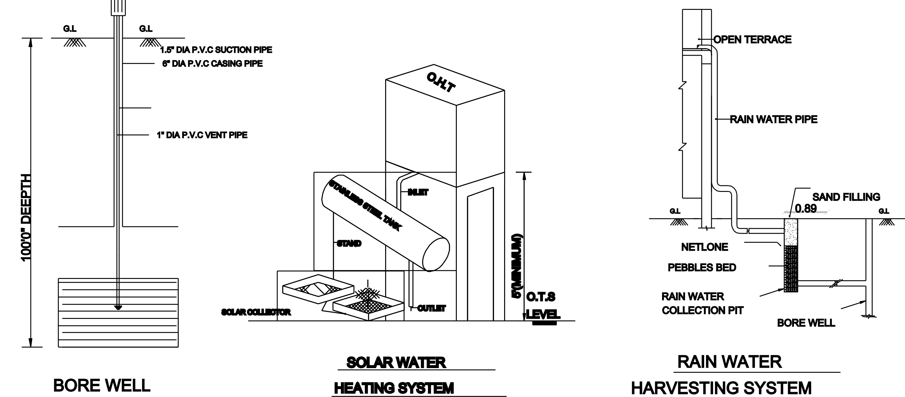
WATER TANK CAPACITY - 1000 LITRES
