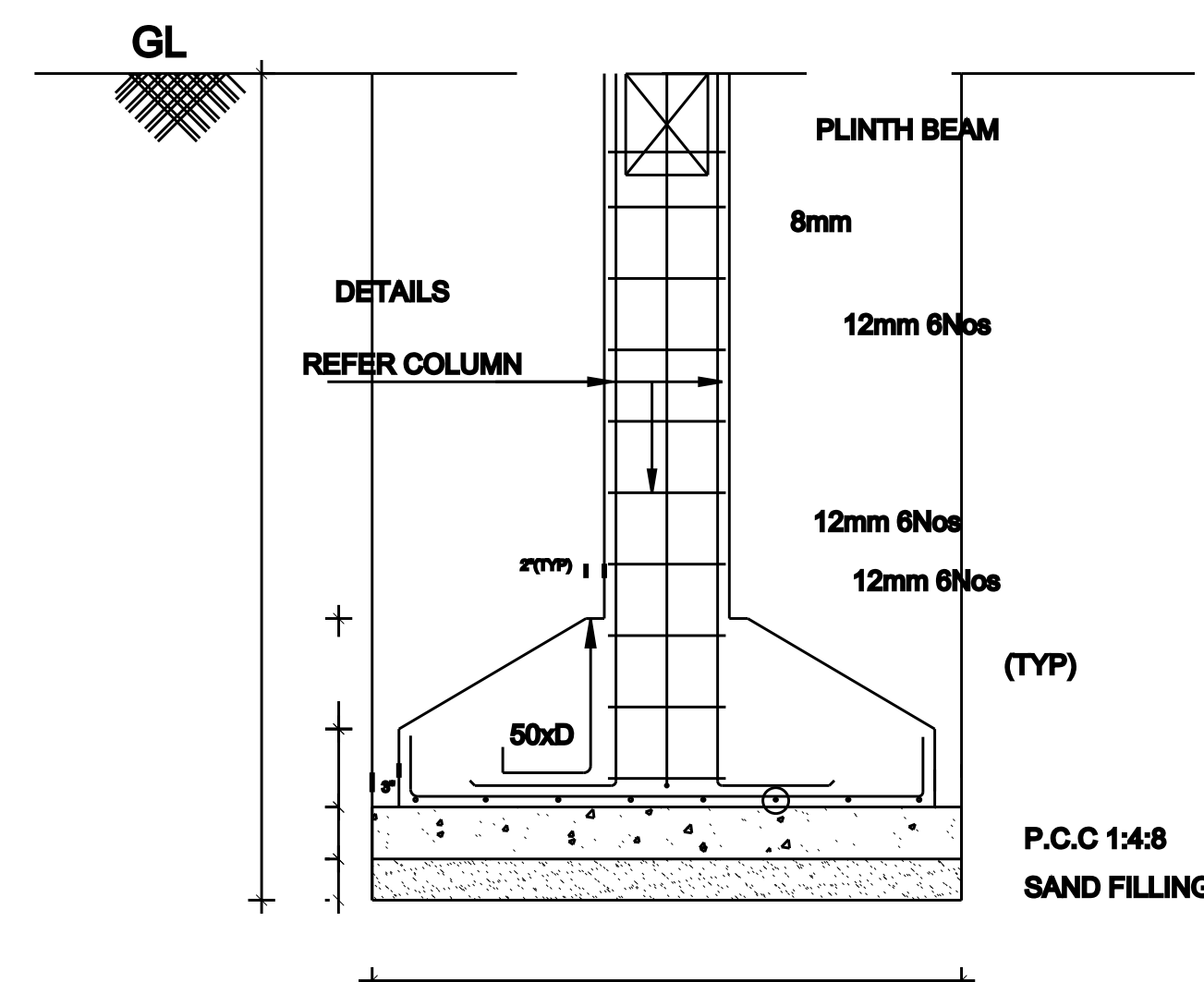
FOUNDATION DETAILS
