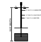
BORE WELL DETAILS
