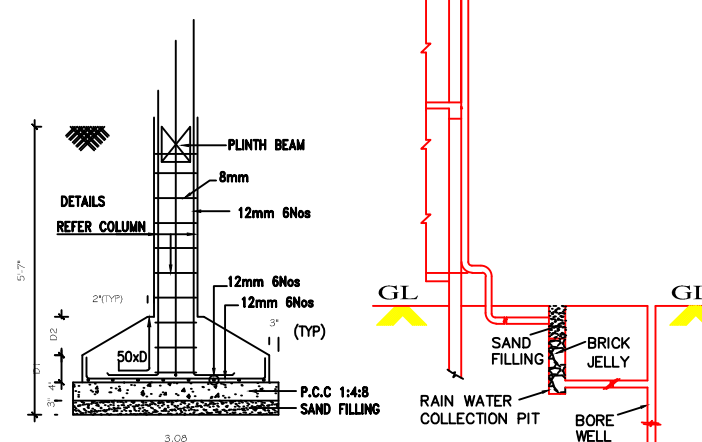
FOUNDATION DETAILS
