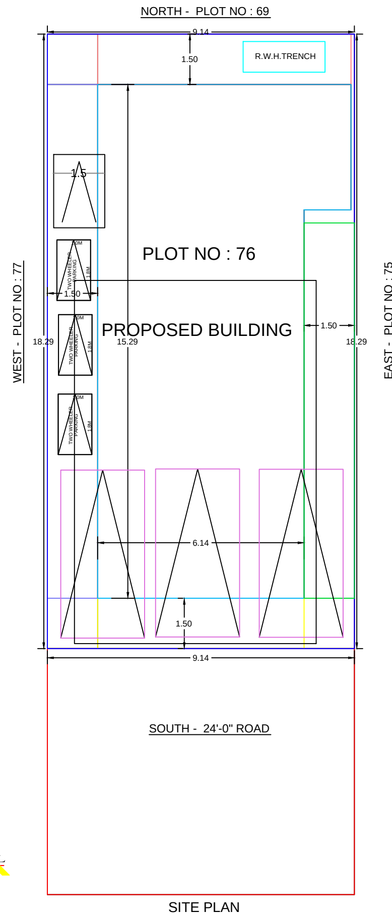
SITE PLAN
