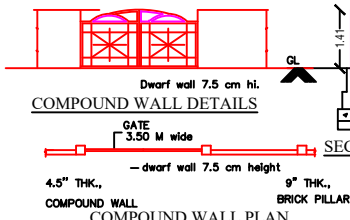
COMPOUND WALL DETAILS COMPOUND WALL PLAN
