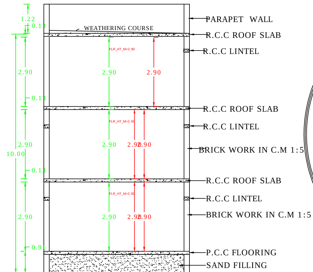
SECTION
