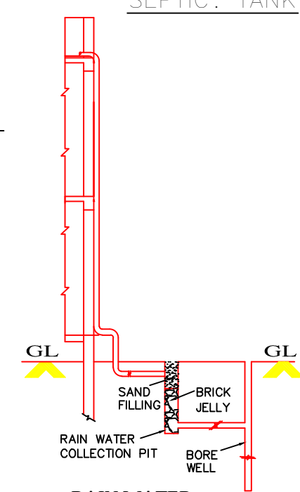
RAIN WATER HARVESTING SYSTEM
