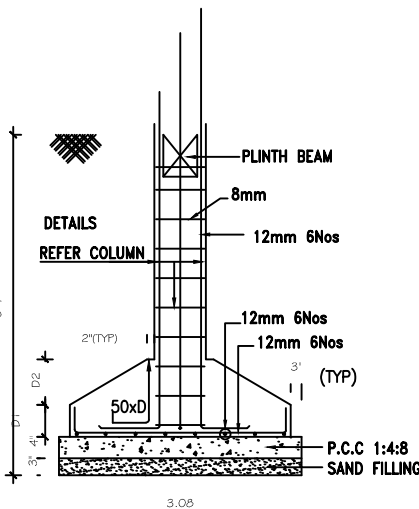
FOUNDATION DETAILS
