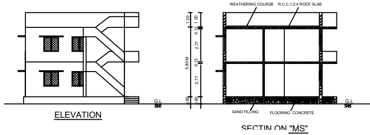
SECTION ON "MS"
