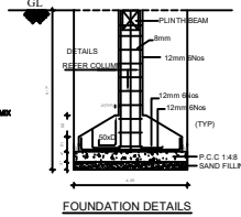
FOUNDATION DETAILS
