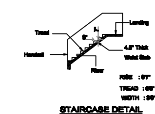
STAIRCASE DETAIL
