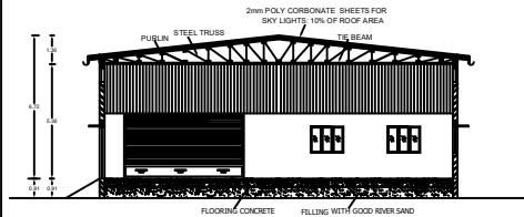
SECTION ON "MS"
