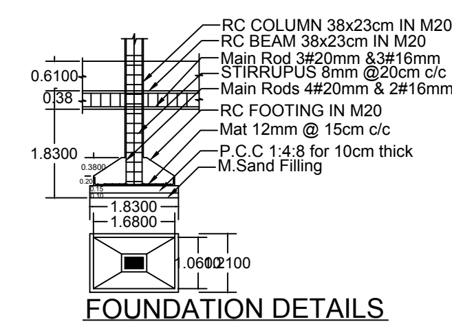
FOUNDATION DETAILS
