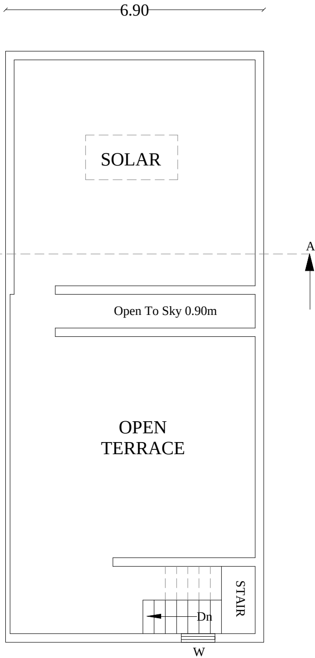
TERRACE FLOOR
