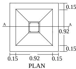
FOUNDATION DETAILS
