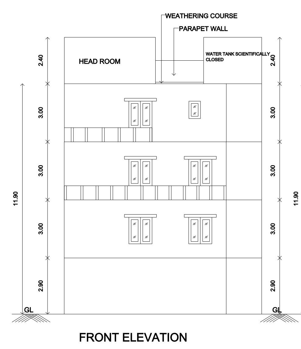
FRONT ELEVATION
