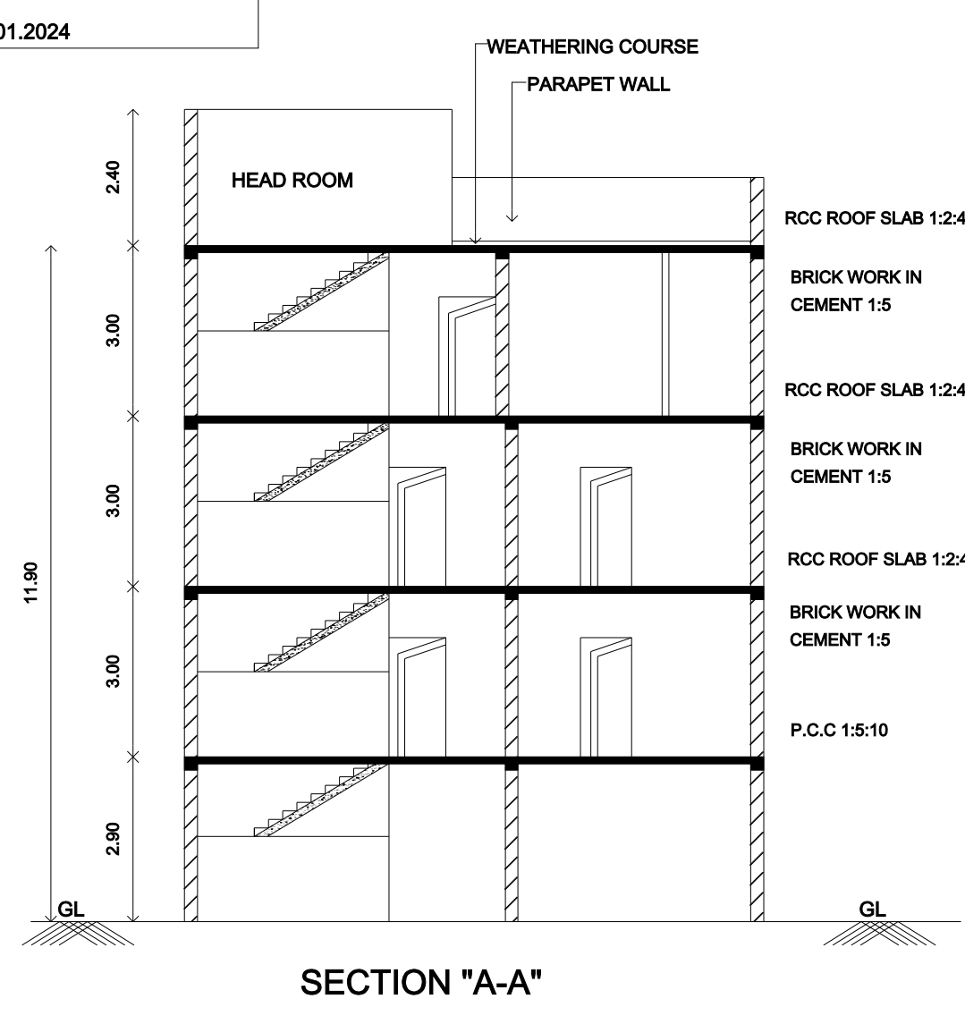
SECTION "A-A"
