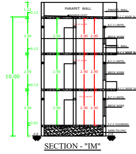
SECTION - "IM"
