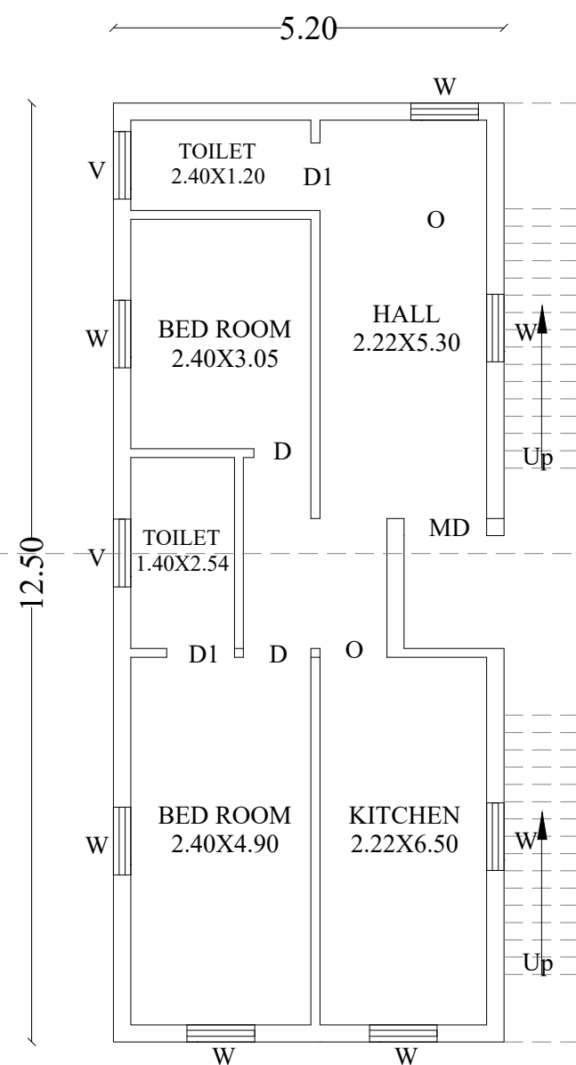
FIRST FLOOR
