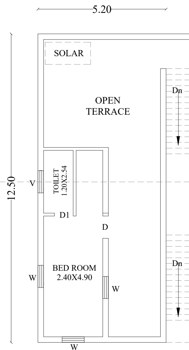
SECOND FLOOR
