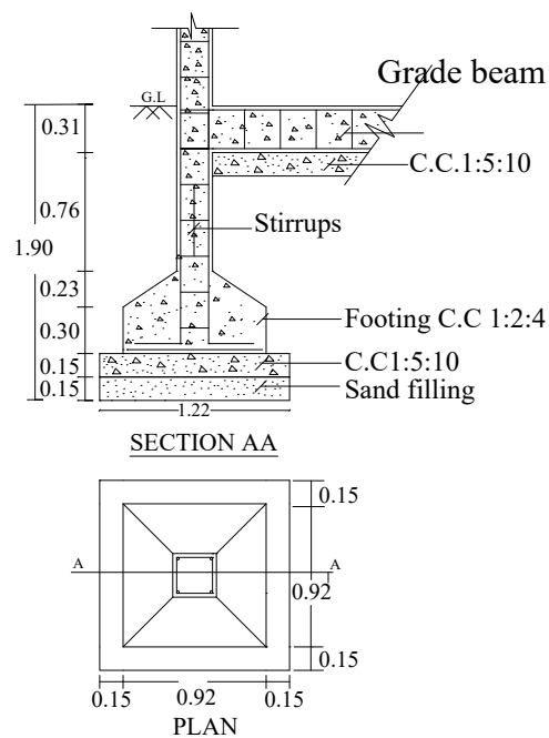
FOUNDATION DETAILS
