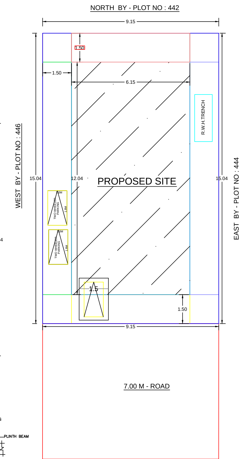
SITE PLAN
