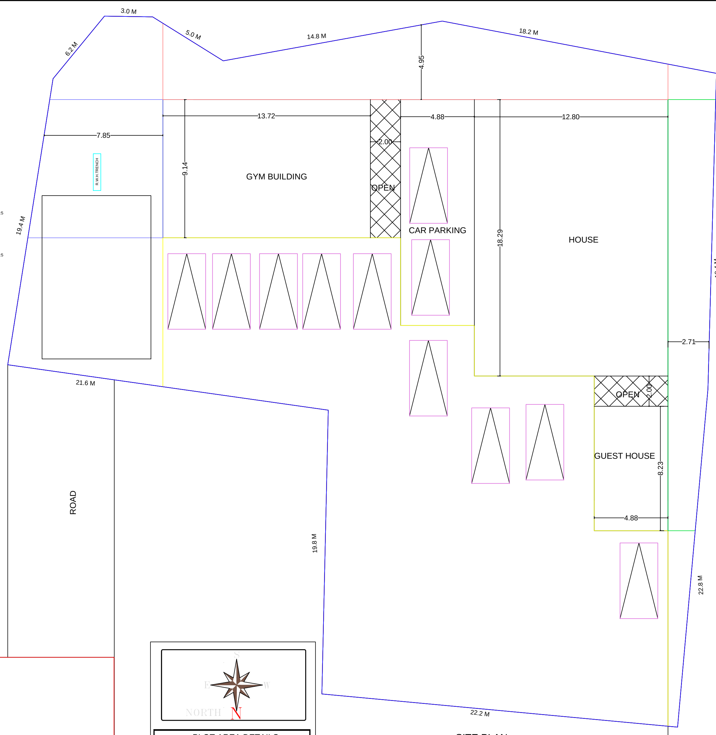
SITE PLAN
