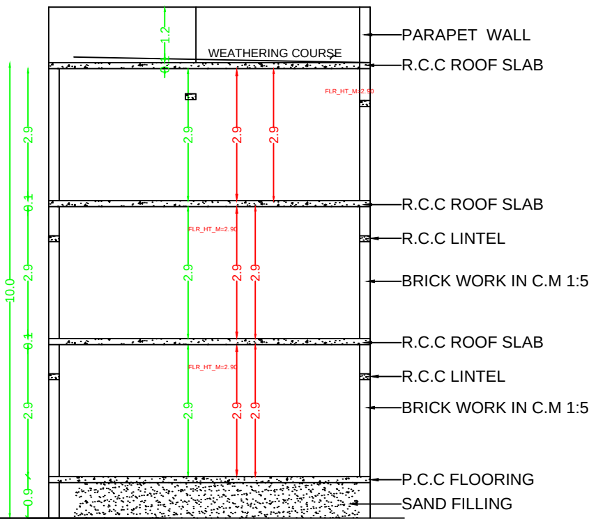
SECTION
