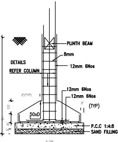
FOUNDATION DETAILS
