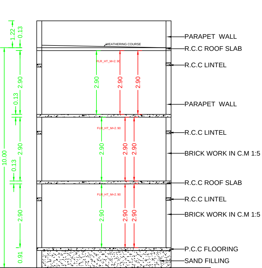
SECTION
