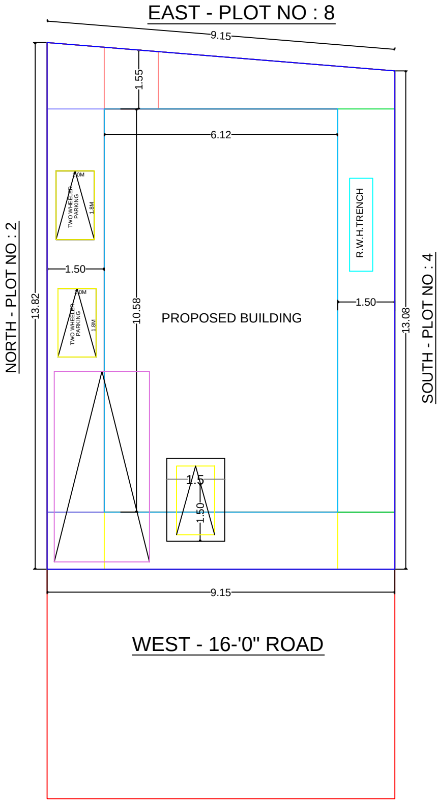
SITE PLAN
