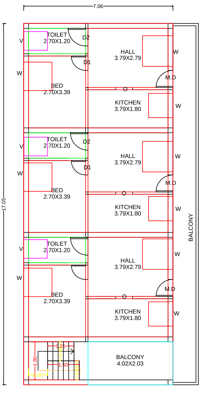
PROPOSED SECODN FLOOR PLAN
