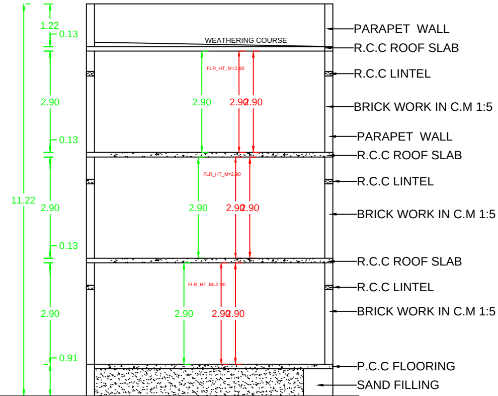
SECTION
