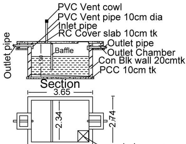
Plan SEPTIC TANK DETAILS
