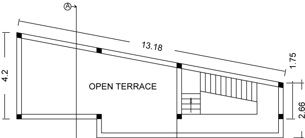
PROPOSED TERRACE FLOOR PLAN
