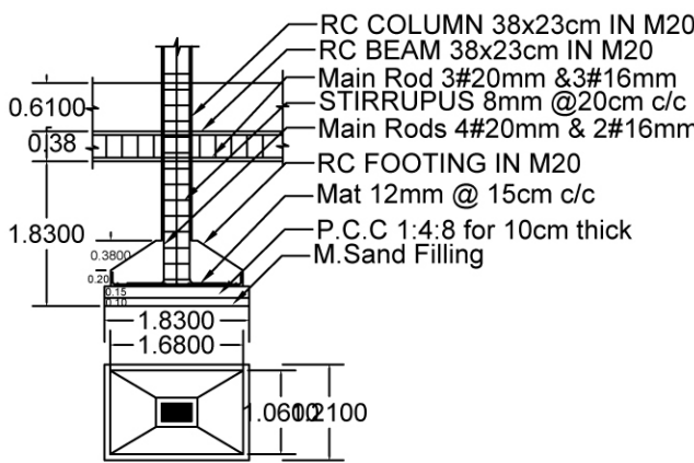
FOUNDATION DETAILS
