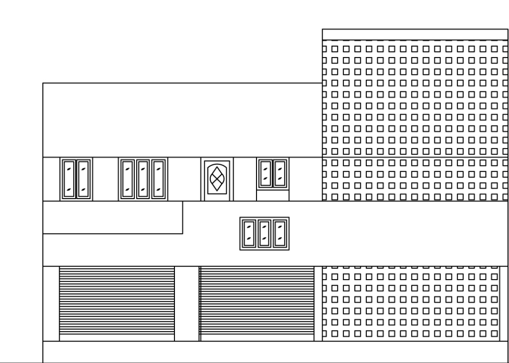
FRONT ELEVATION
