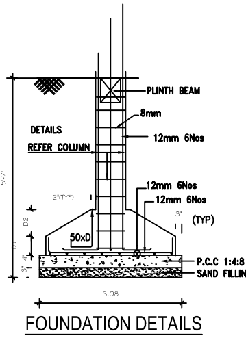
FOUNDATION DETAILS
