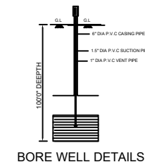
BORE WELL DETAILS
