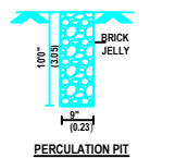
PERCOLATION PIT
