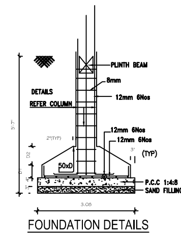
FOUNDATION DETAILS
