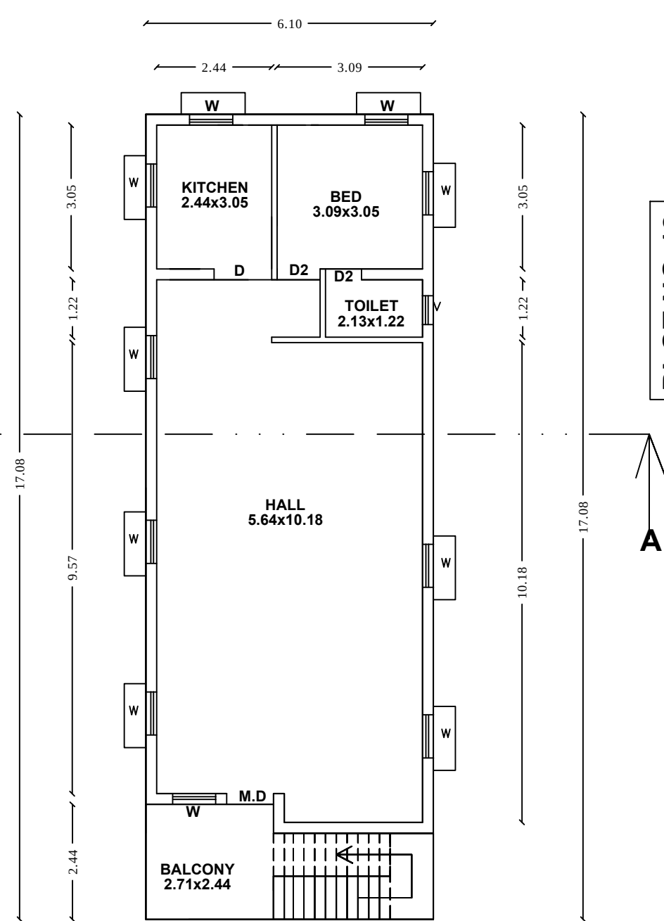
1st & 2nd FLOOR PLAN
