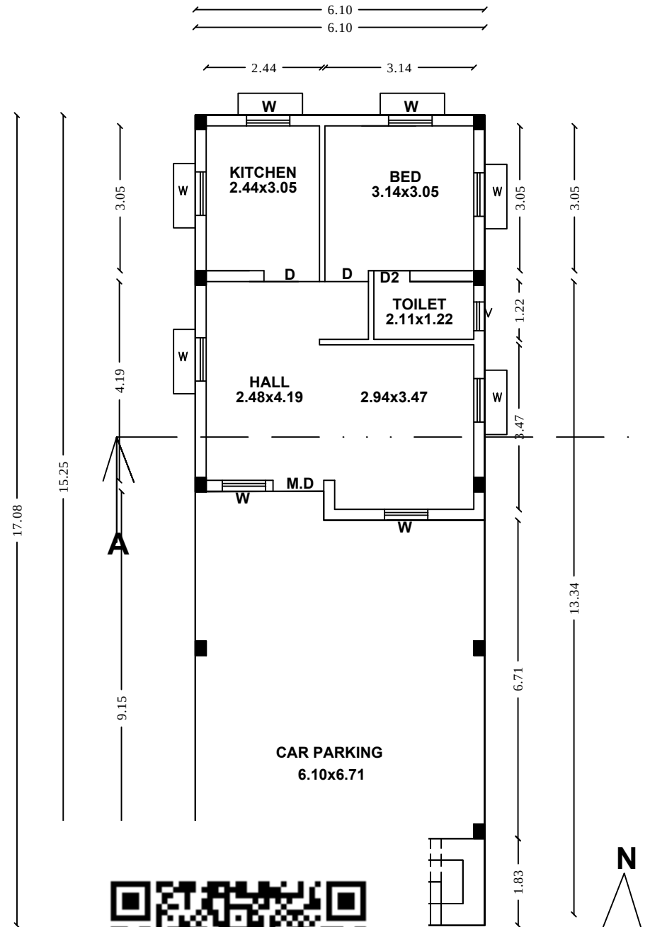
PLAN
