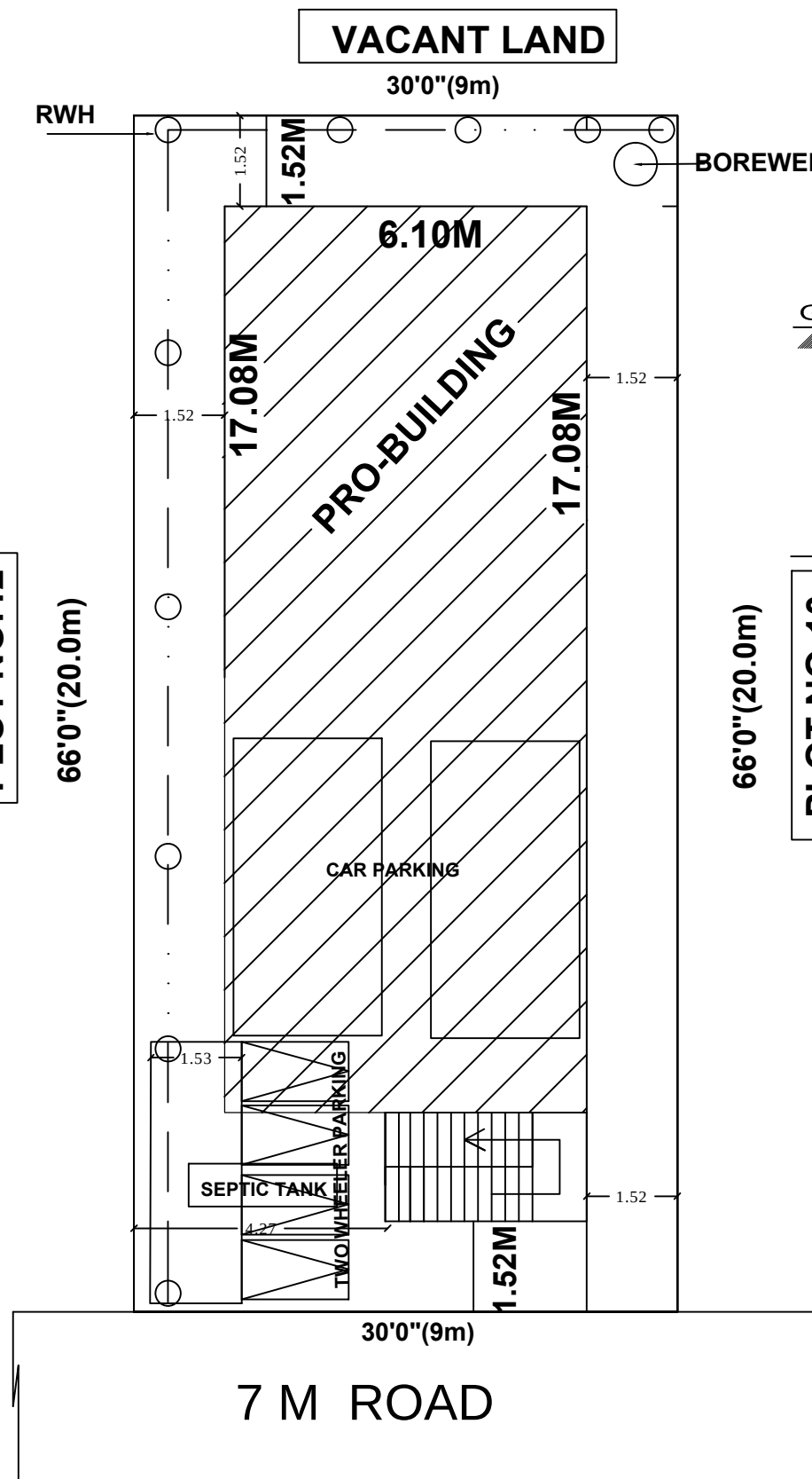
SITE PLAN
