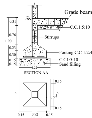
FOUNDATION DETAILS
