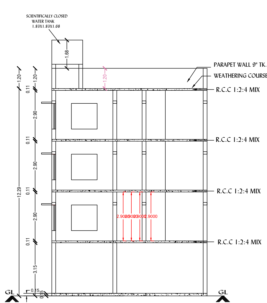
SECTION : "A-A"
