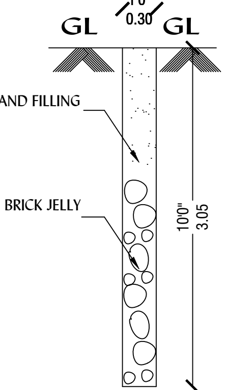
PERCOLATION PIT
