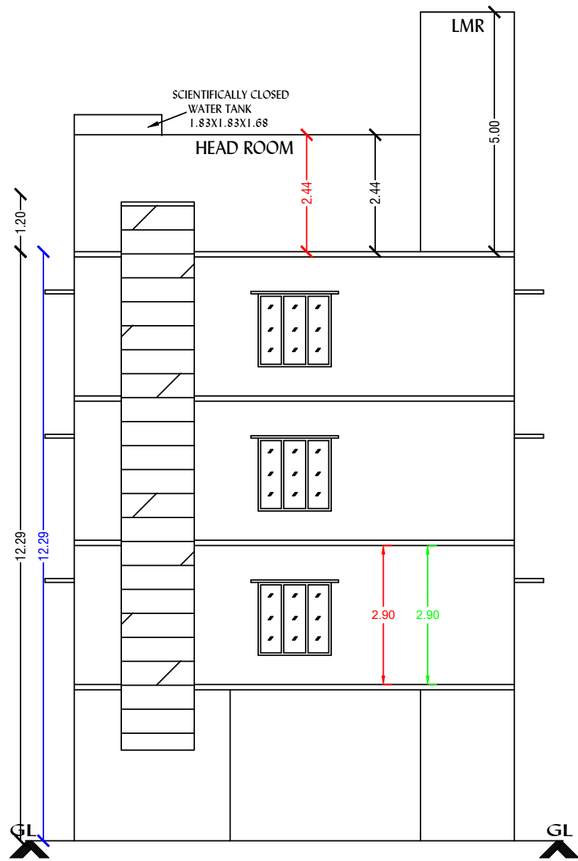
FRONT ELEVATION
