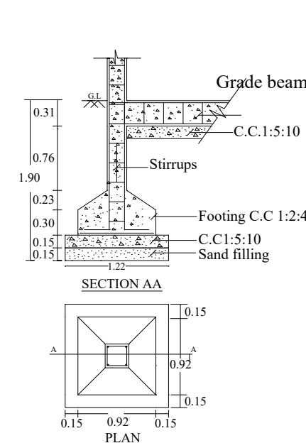
FOUNDATION DETAILS
