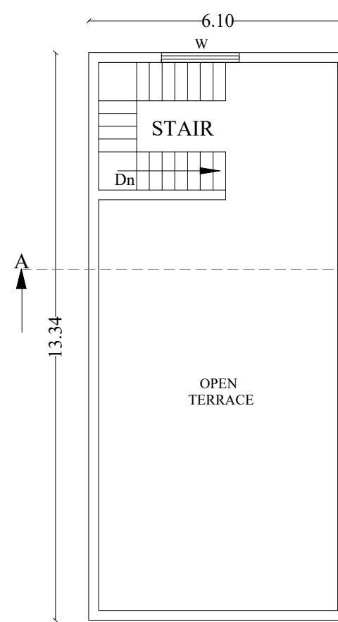
TERRACE FLOOR
