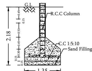
FOUNDATION DETAILS SCALE 1:50
