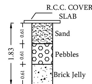
SECTION
