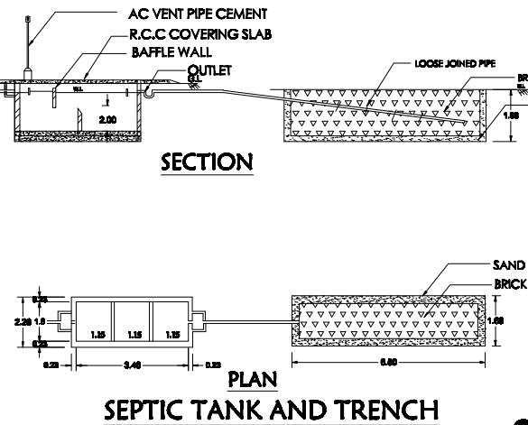
SECTION SEPTIC TANK AND TRENCH
