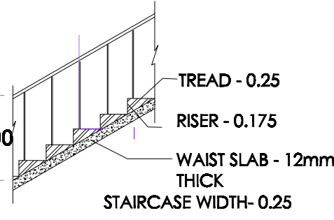
STAIR CASE DETAIL
