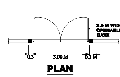
PLAN COMPOUND WALL DETAIL
