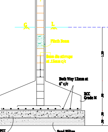
SECTION OF FOOTING
