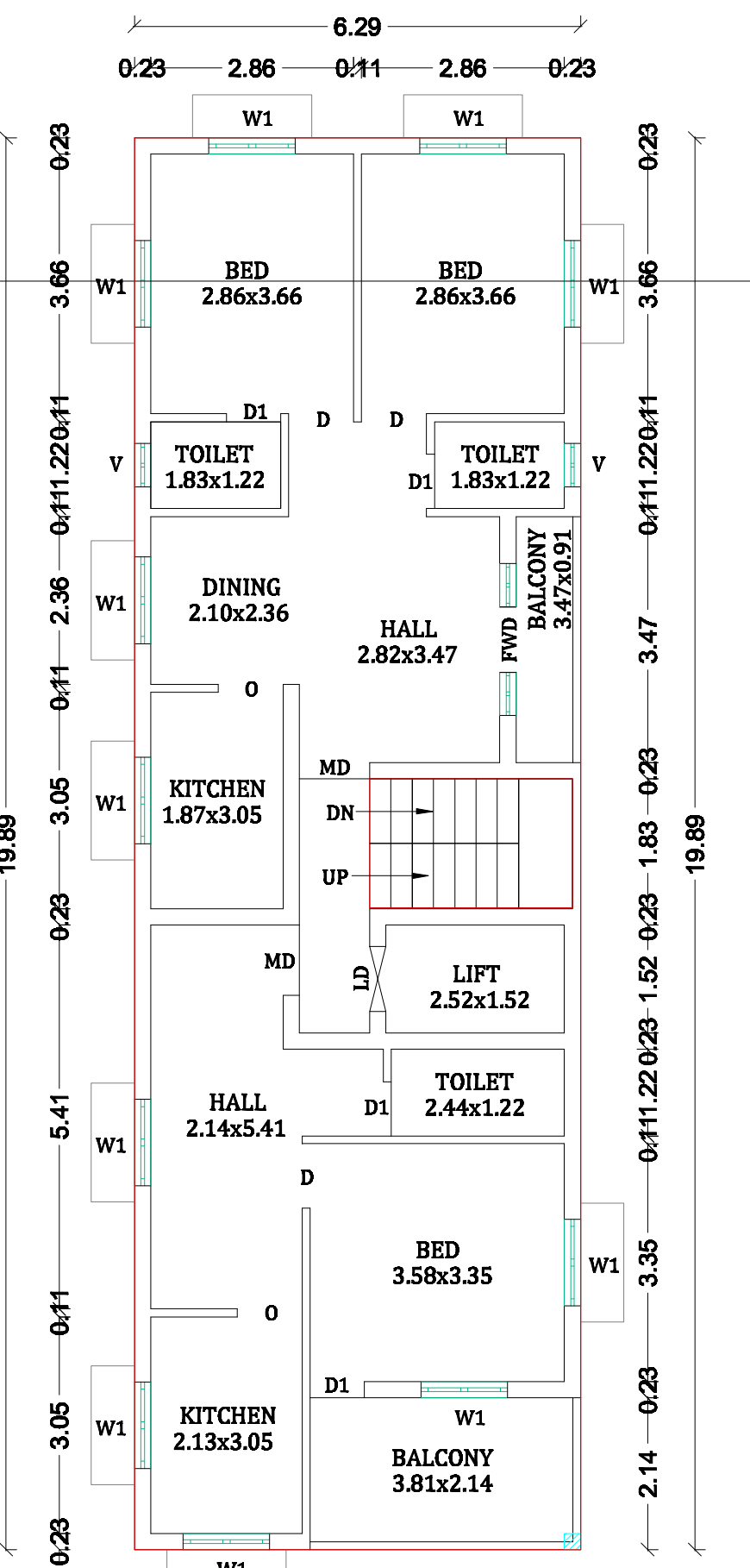
TYPICAL FLOOR PLAN (FIRST & SECOND FLOOR PLAN)
