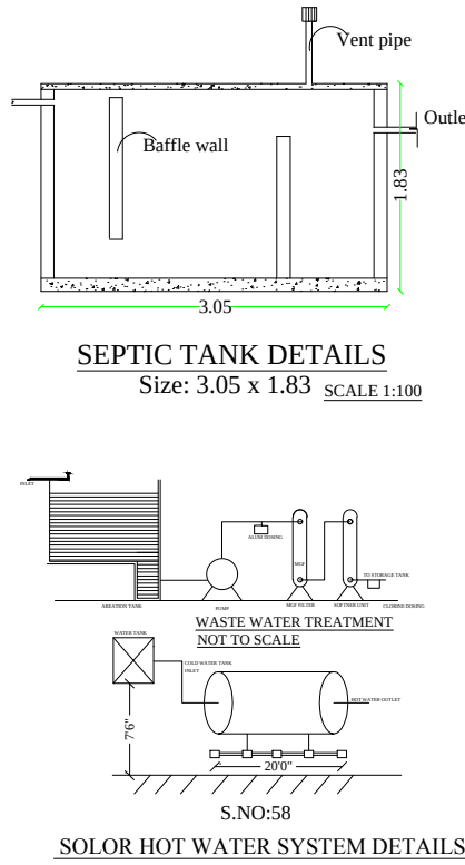
SEPTIC TANK DETAILS
