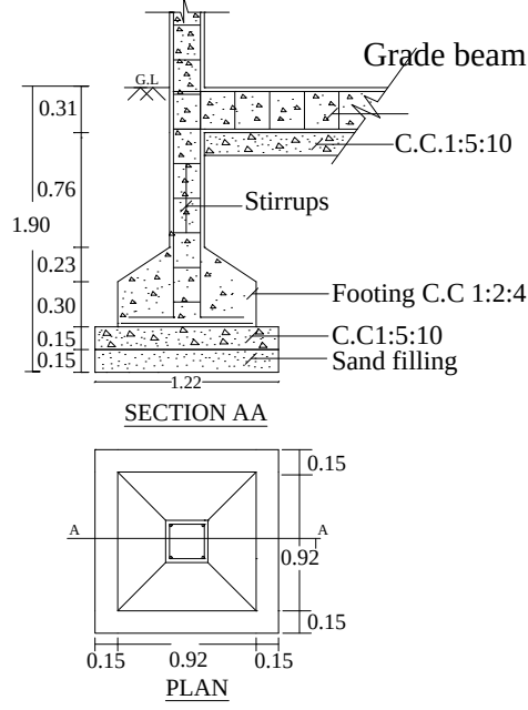
FOUNDATION DETAILS
